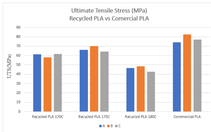
Fig. 19 Diagram of the Ultimate Tensile Stress of Recycled PLA Filament vs Commercial PLA Filament
