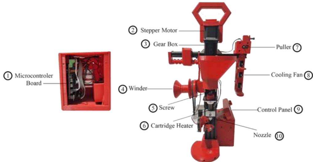
Fig. 2 Extrusion Machine
