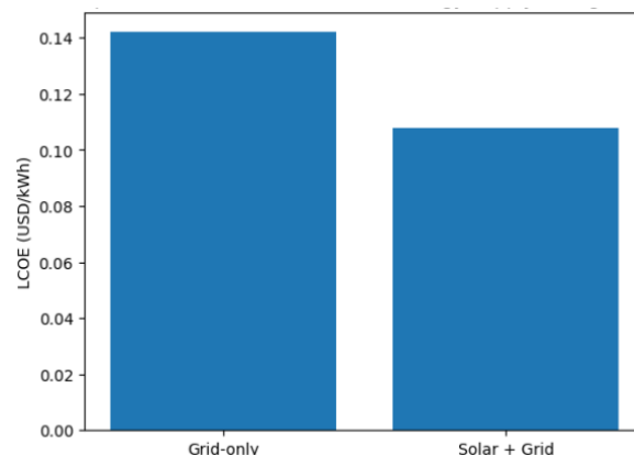
Fig. 1. Comparison of Levelized Cost of Energy (LCOE) between grid-only and solar-grid hybrid energy supply configurations for electric heavy equipment
